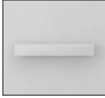
C – Cubic
